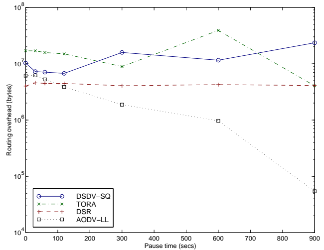
(b) Routing overhead in bytes.
